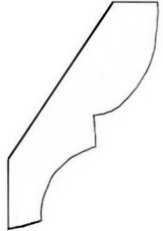
#W-10B 5/8" x 2 3/4"
