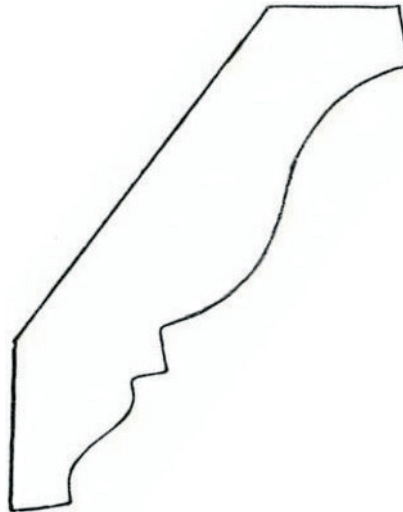
#369 3/4" x 3.26"
