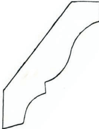
#370 5/8" x 2 13/16"
