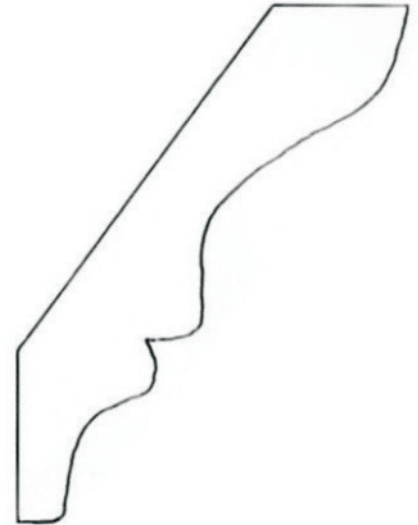
#277 3/4" x 3 1/2"
