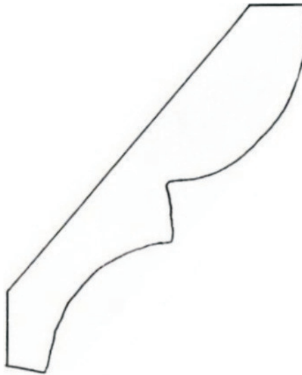
#W-9B 3/4" x 3 1/2"
